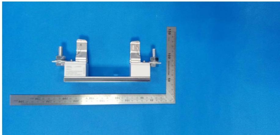
Picture 15 Fuse-holder DNF2-1
