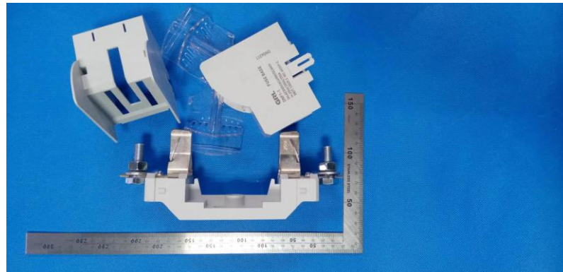
Picture 13 Fuse-holder DNF1-1
